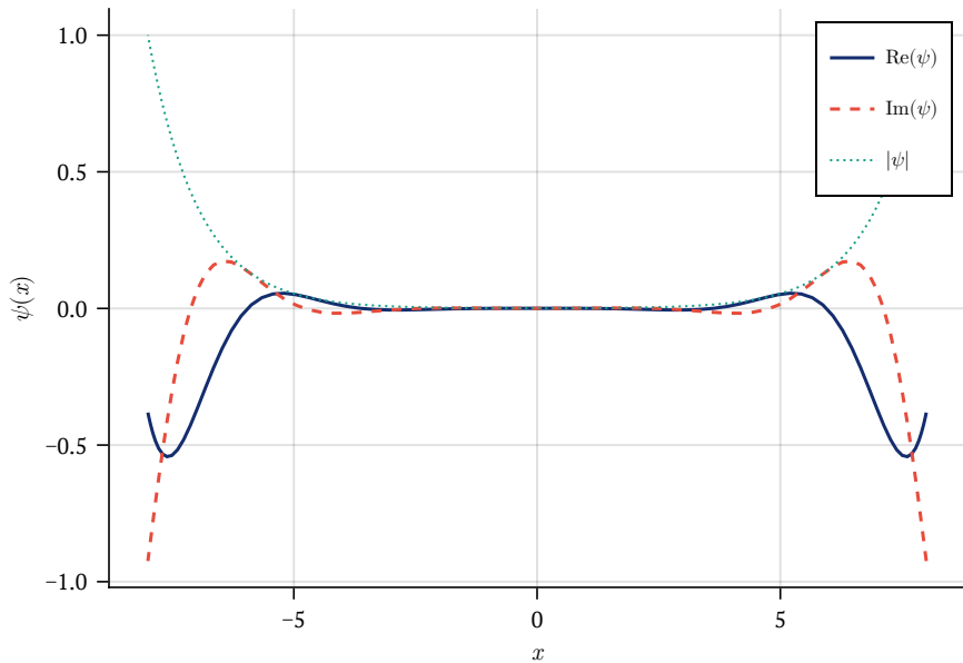
First overtone: \omega = 1.3424-0.9723i
