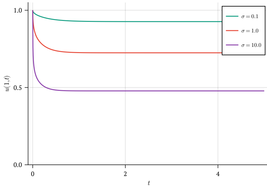
Boundary temperature at radiating end
