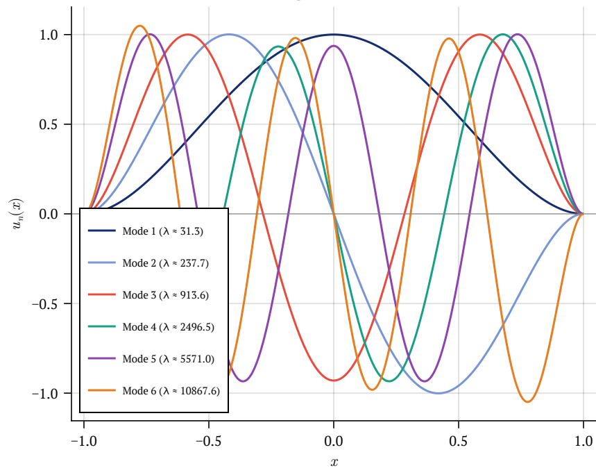
First 6 eigenmodes (N = 30)
