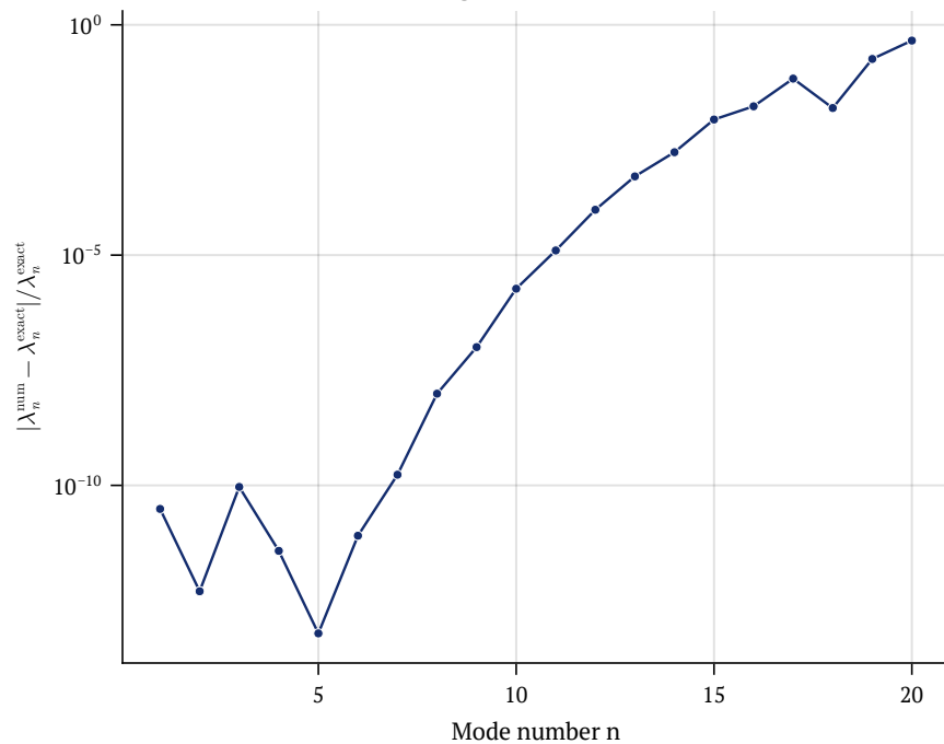
Relative eigenvalue error (N = 30)
