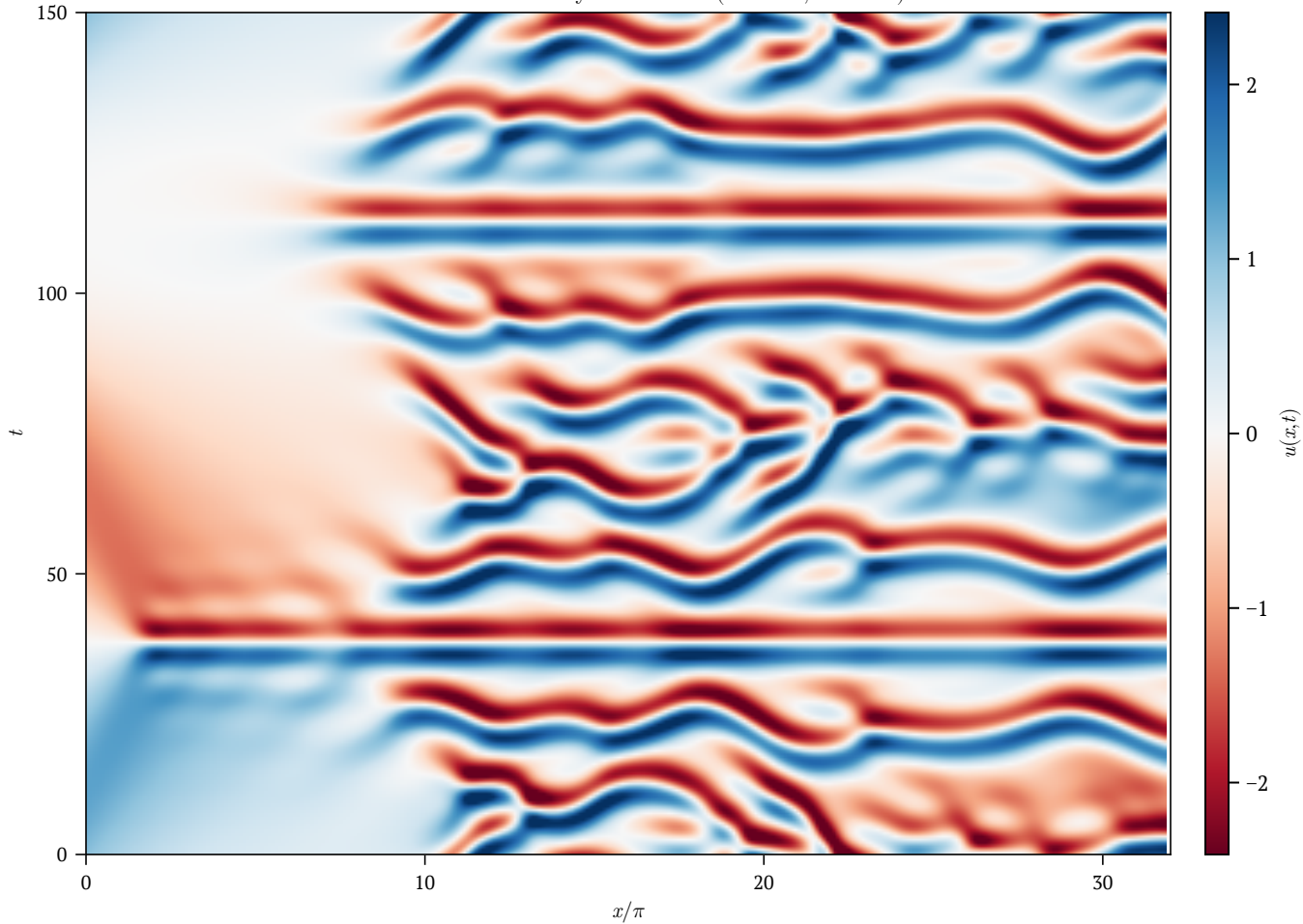
Kuramoto--Sivashinsky : ETDRK4 ( L = 32\pi , N = 256 )
