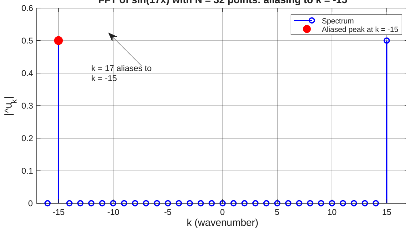
FFT of \sin(17x) with N = 32 points: aliasing to k = -15
