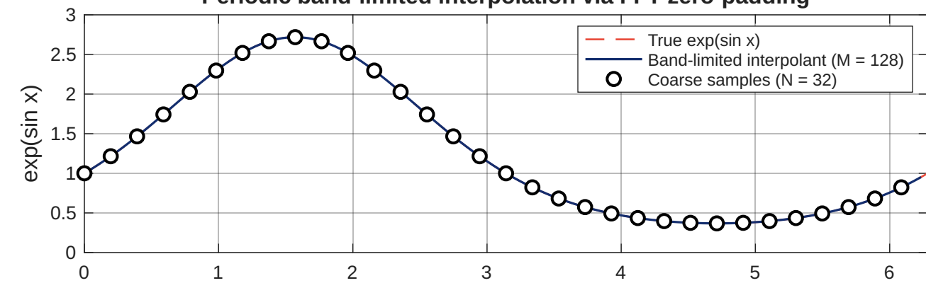
Periodic band-limited interpolation via FFT zero-padding
