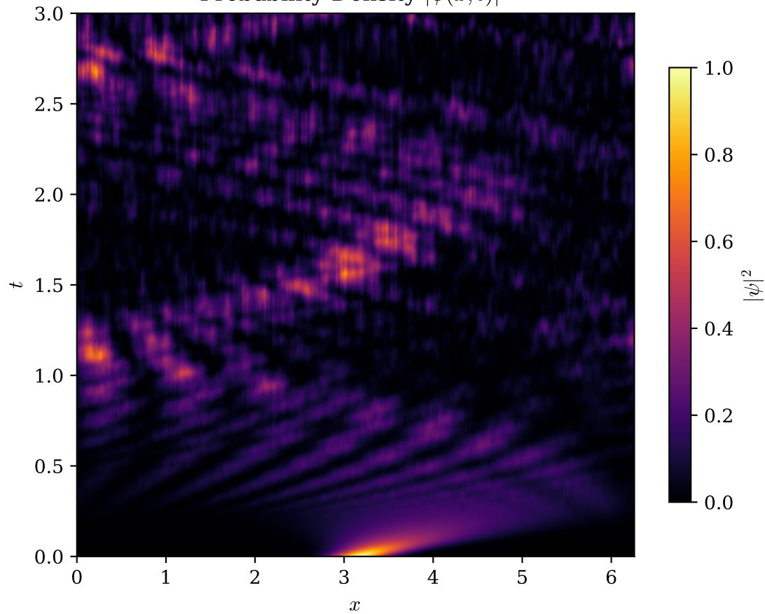
Probability Density |\psi(x, t)|^2
