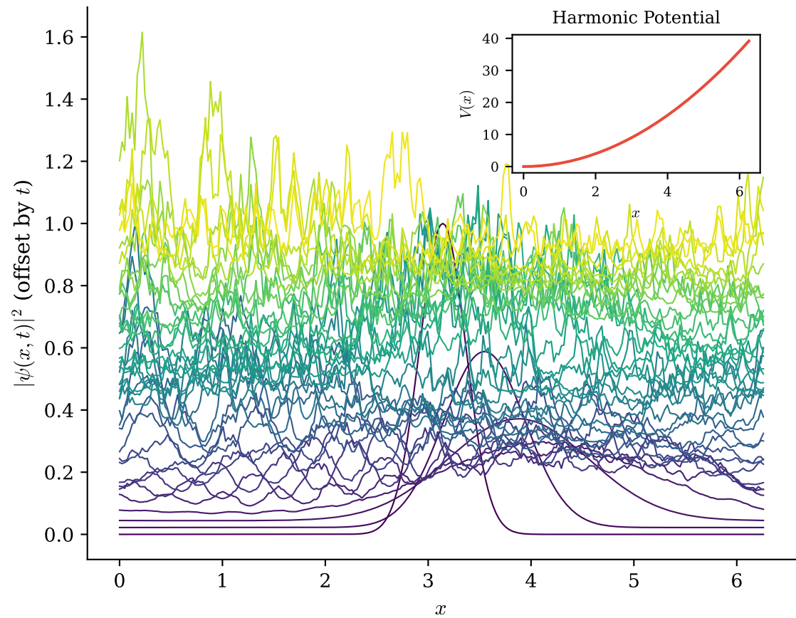
Waterfall View: |\psi|^2 Evolution
