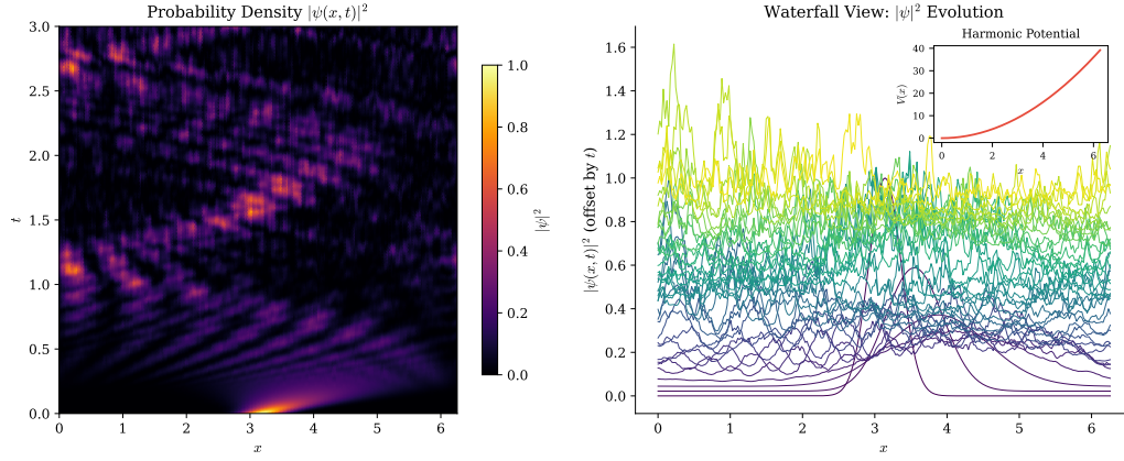
Figure 65: Solution of the Schrödinger equation Equation 152 with harmonic potential using Strang splitting. Left: space-time evolution of the probability density |\psi(x,t)|^2 showing the oscillatory dynamics of a Gaussian wavepacket in the harmonic trap. Right: waterfall plot of |\psi(x,t)|^2 at selected times.
