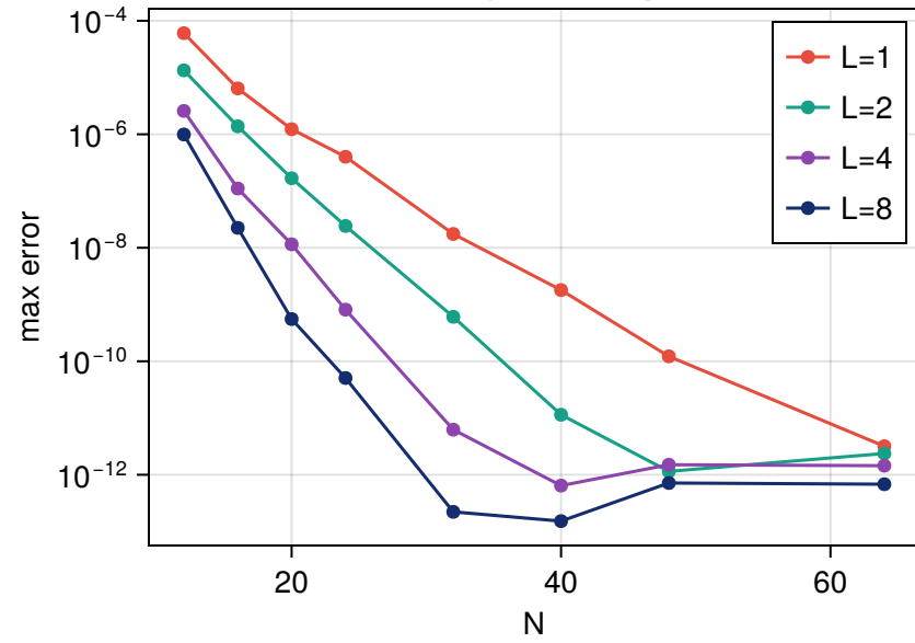
(c) Algebraic map
