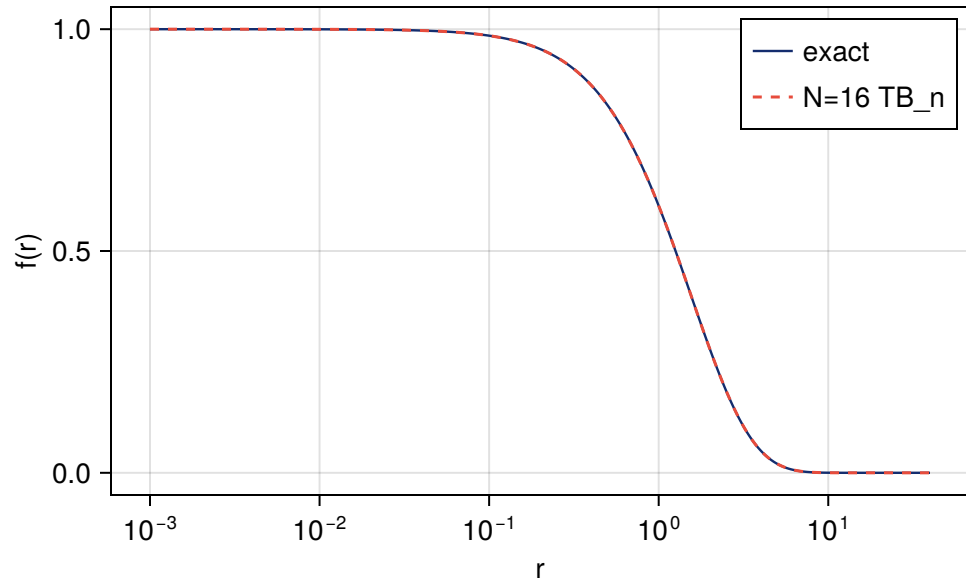
(a) r K_1(r) and N=16 approximation
