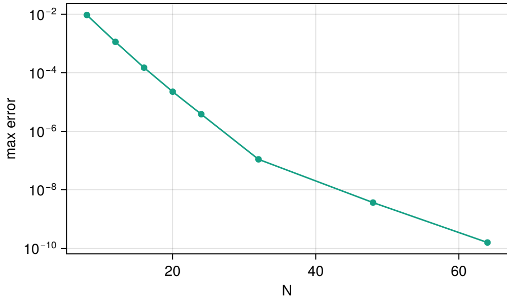
(b) Subgeometric descent, L=4.0
