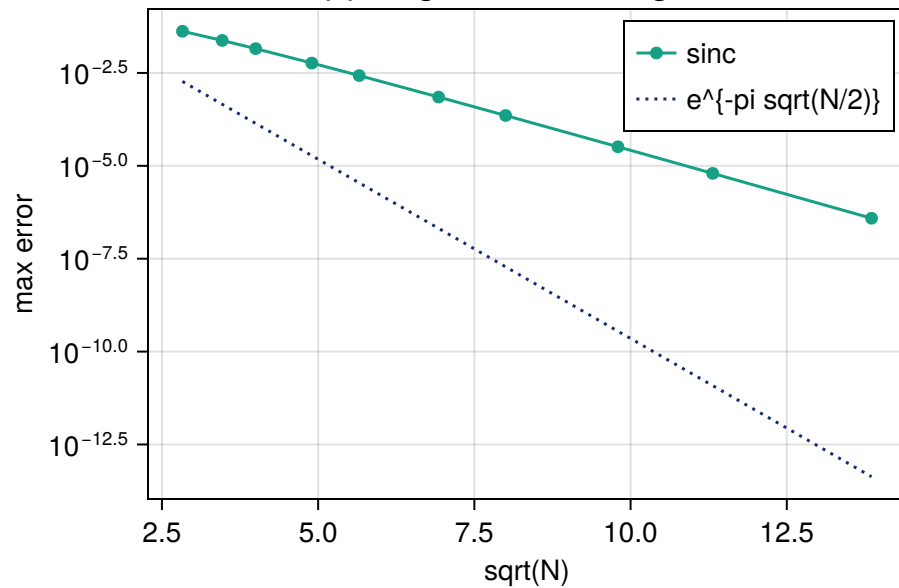
(b) Subgeometric convergence
