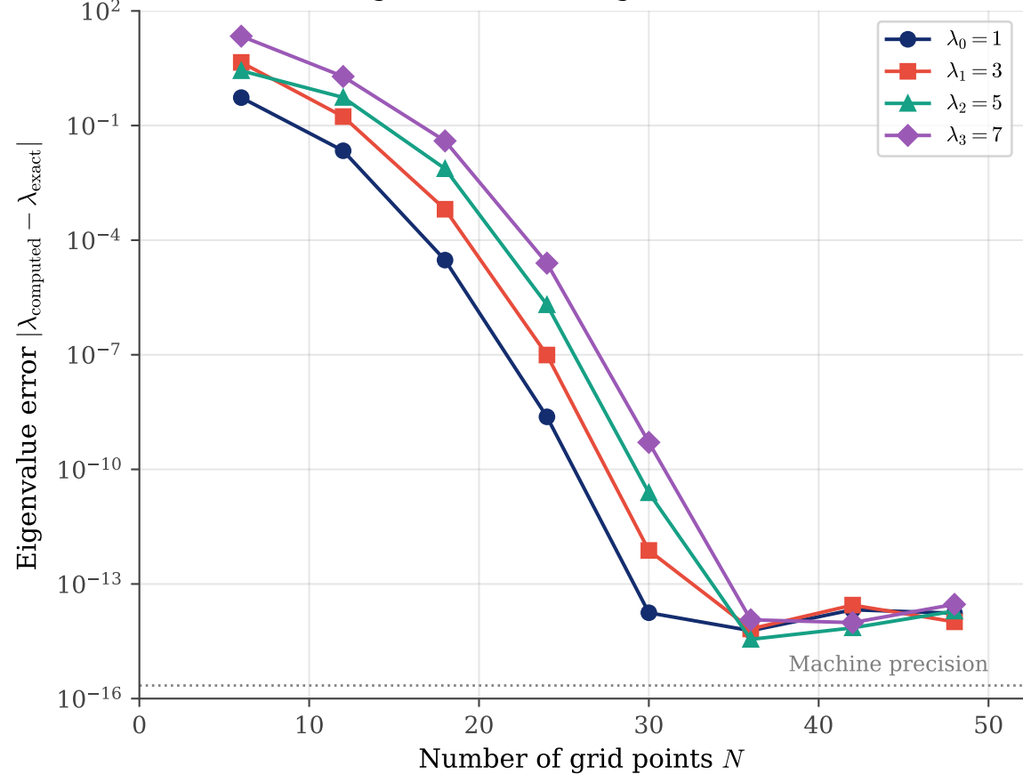
Eigenvalue Convergence ( L = 8.0 )
