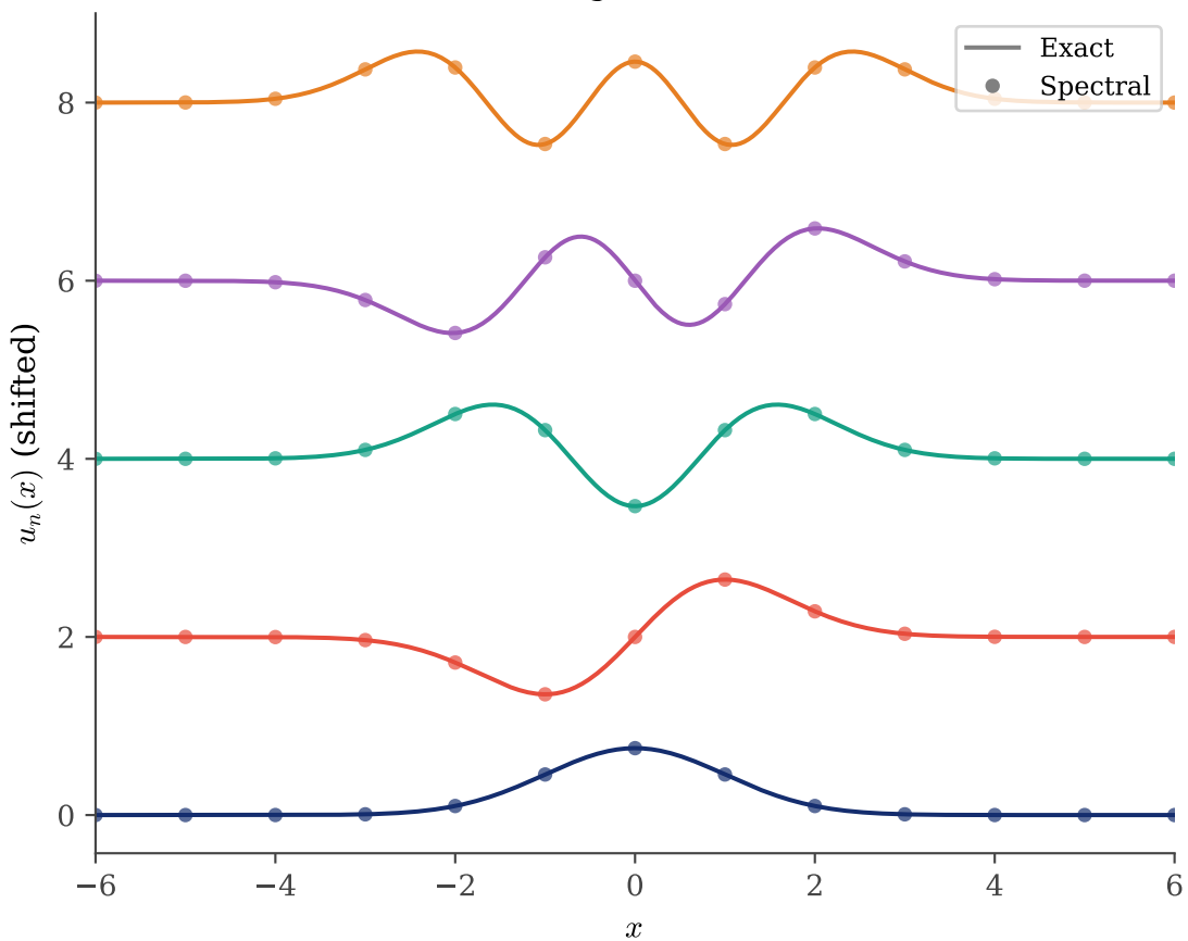
Harmonic Oscillator Eigenfunctions ( N = 64 , L = 8.0 )
