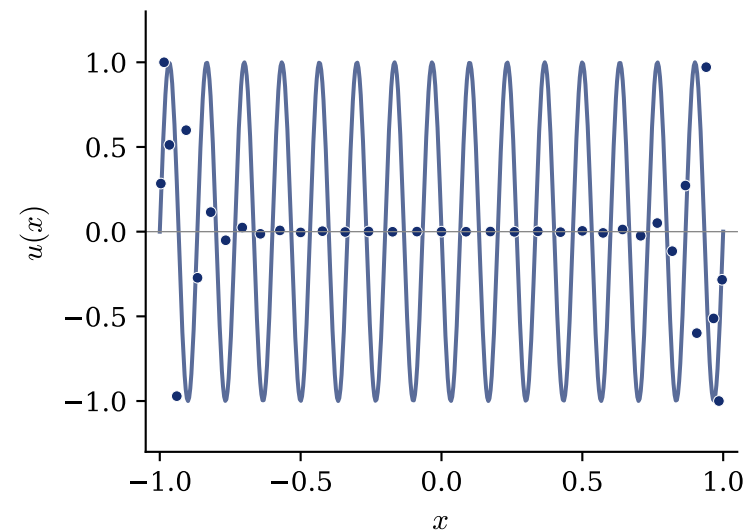
Mode 30: ppw = 2.4, \lambda error = 1.6e+00
