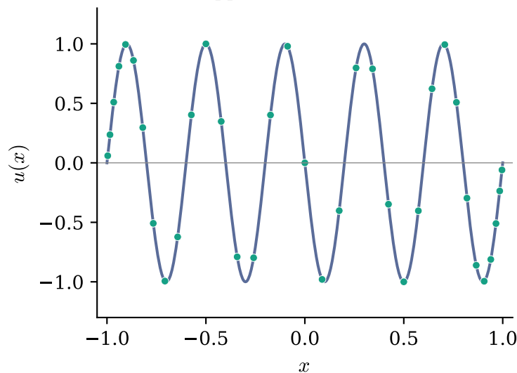
Mode 25: ppw = 2.9, \lambda error = 1.6e-02
