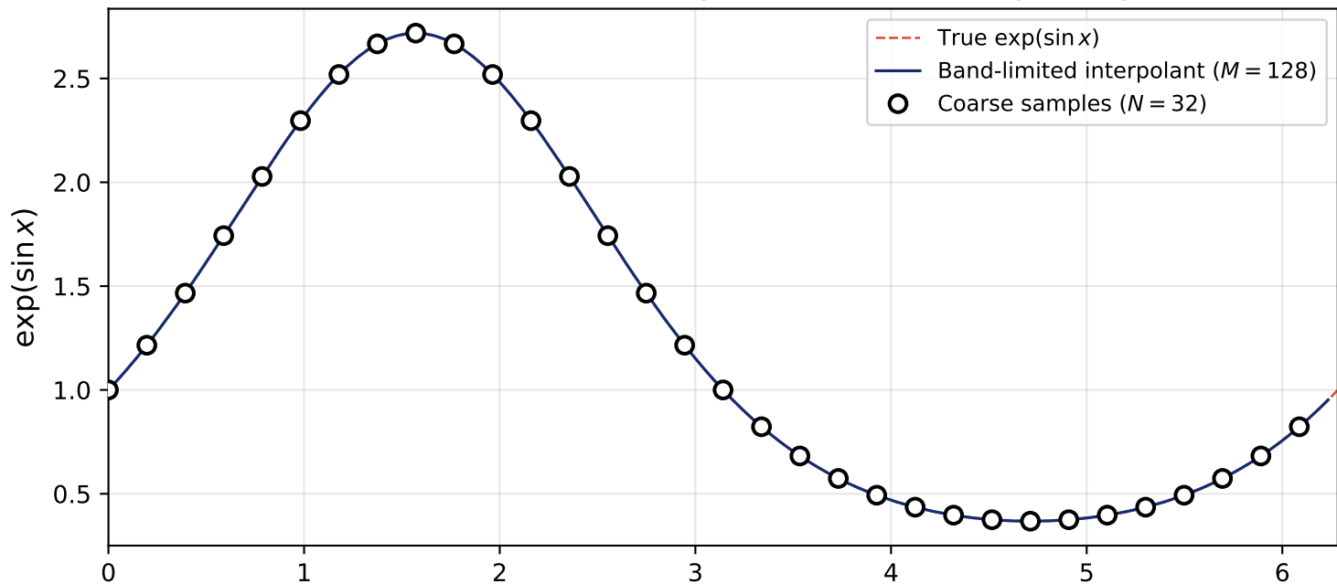
Periodic band-limited interpolation via FFT zero-padding
