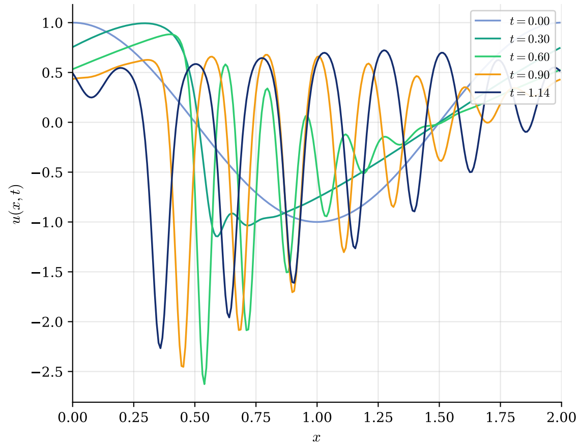
Soliton Train Formation
