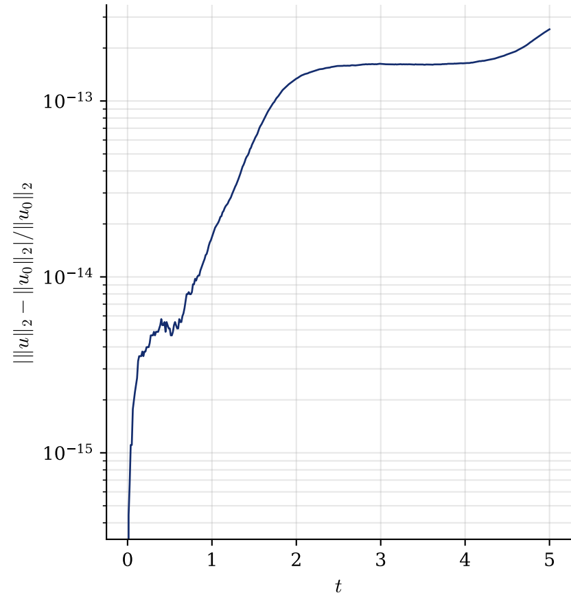
L^2 Norm Conservation
