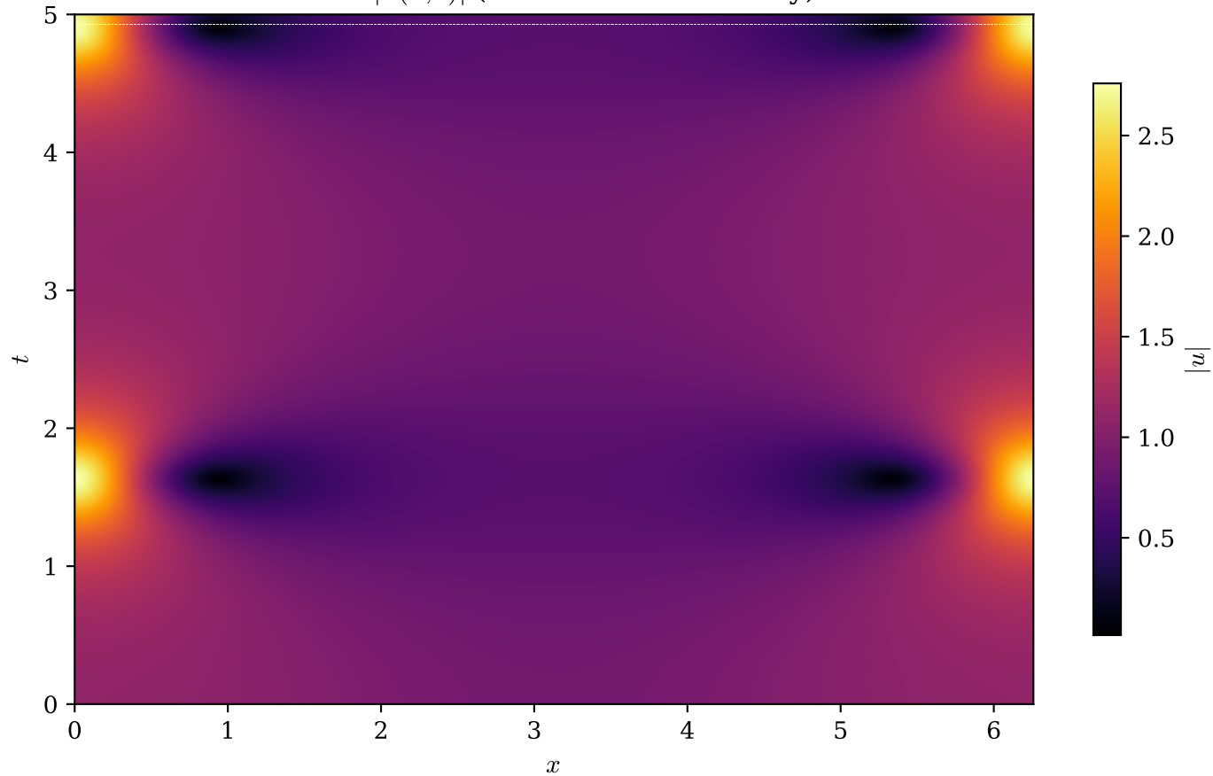
NLS: |u(x, t)| (Modulation Instability)
