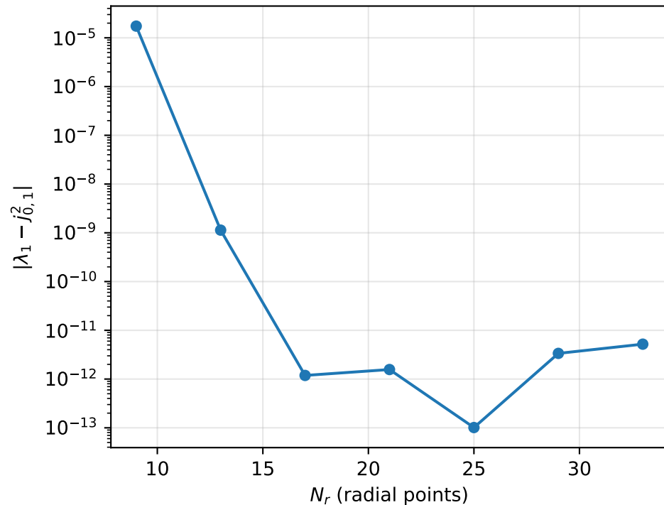
Exponential convergence
