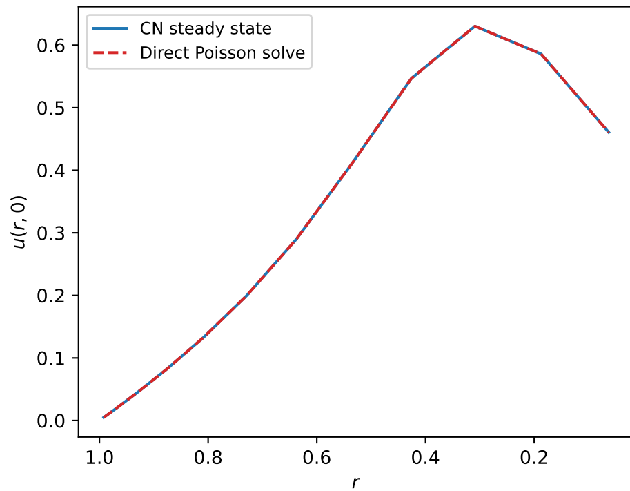
Steady state vs Poisson solution ( \theta = 0 )
