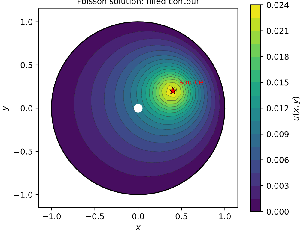
Poisson solution: filled contour
