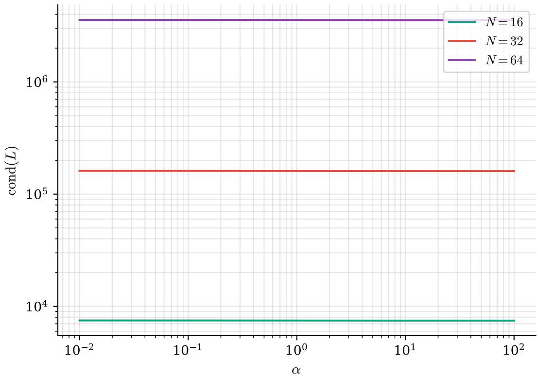
Condition Number vs Robin Parameter \alpha
