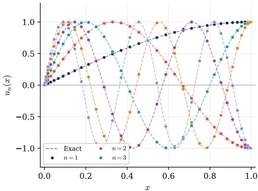
First 6 Eigenmodes ( N = 36 )
