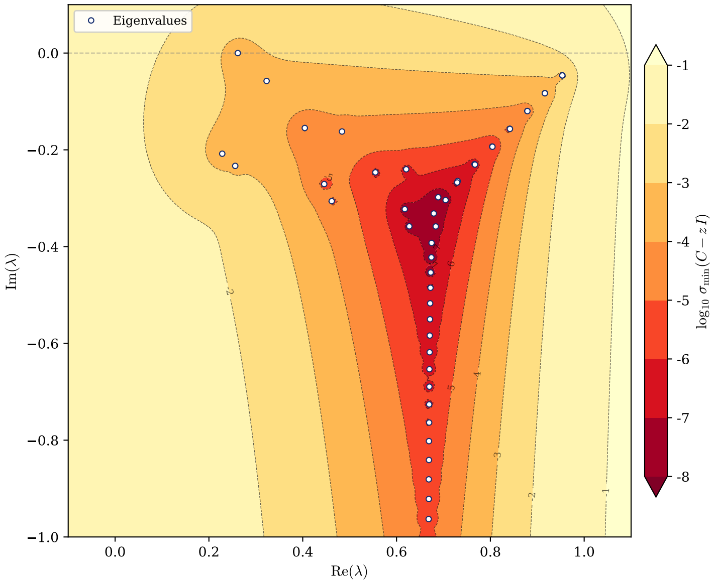
\varepsilon -Pseudospectra of Orr--Sommerfeld: R = 5772 , \alpha = 1 , N = 100
