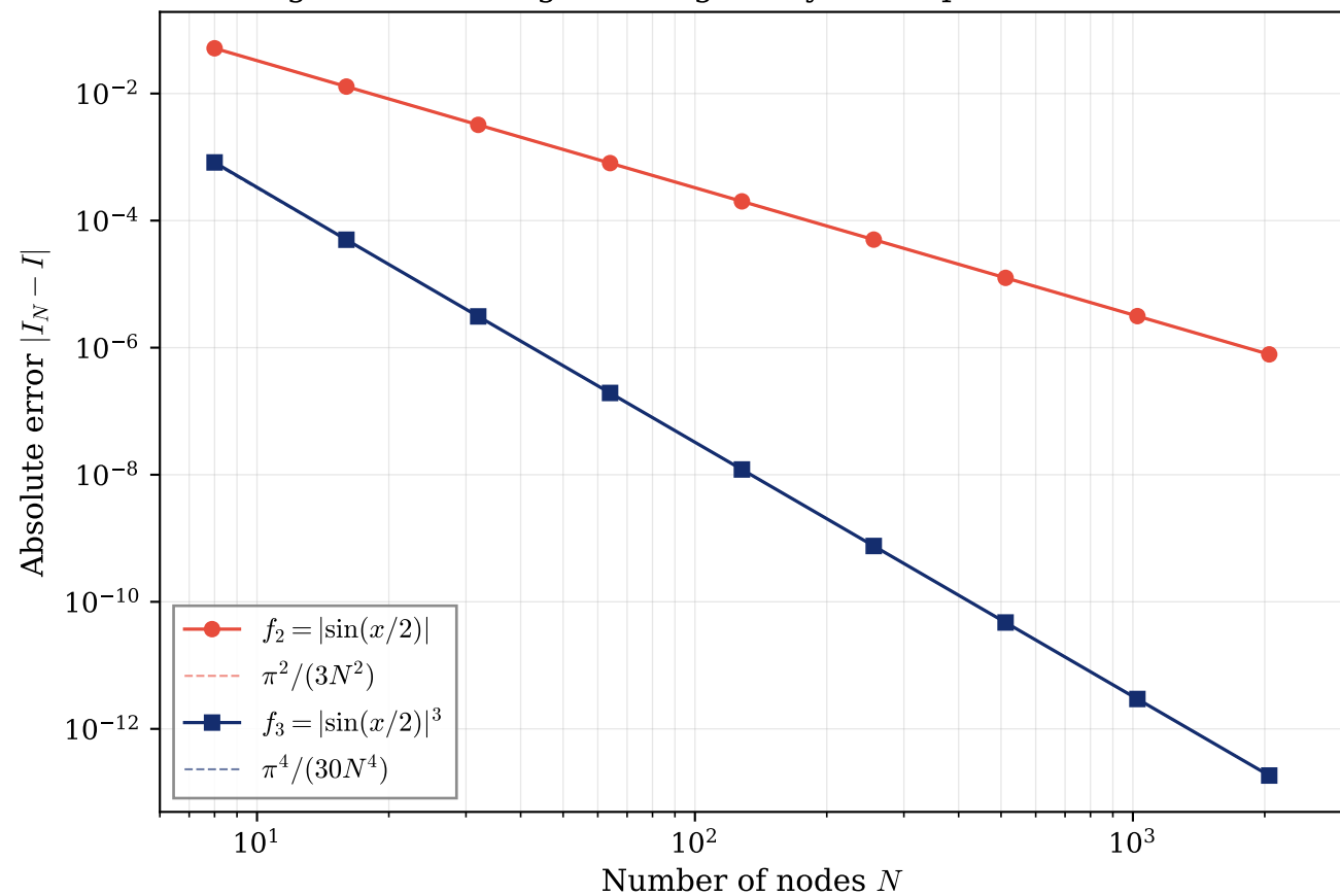
Algebraic convergence: regularity of the periodic extension
