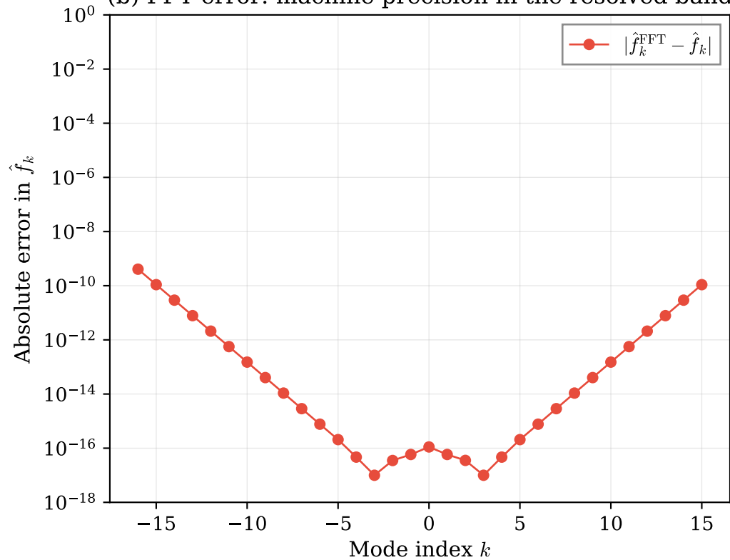
(b) FFT error: machine precision in the resolved band
