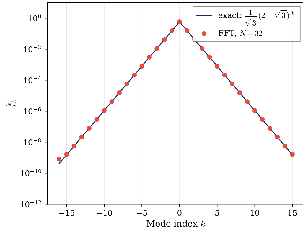
(a) Fourier-coefficient magnitudes for 1/(2 - \cos x)
