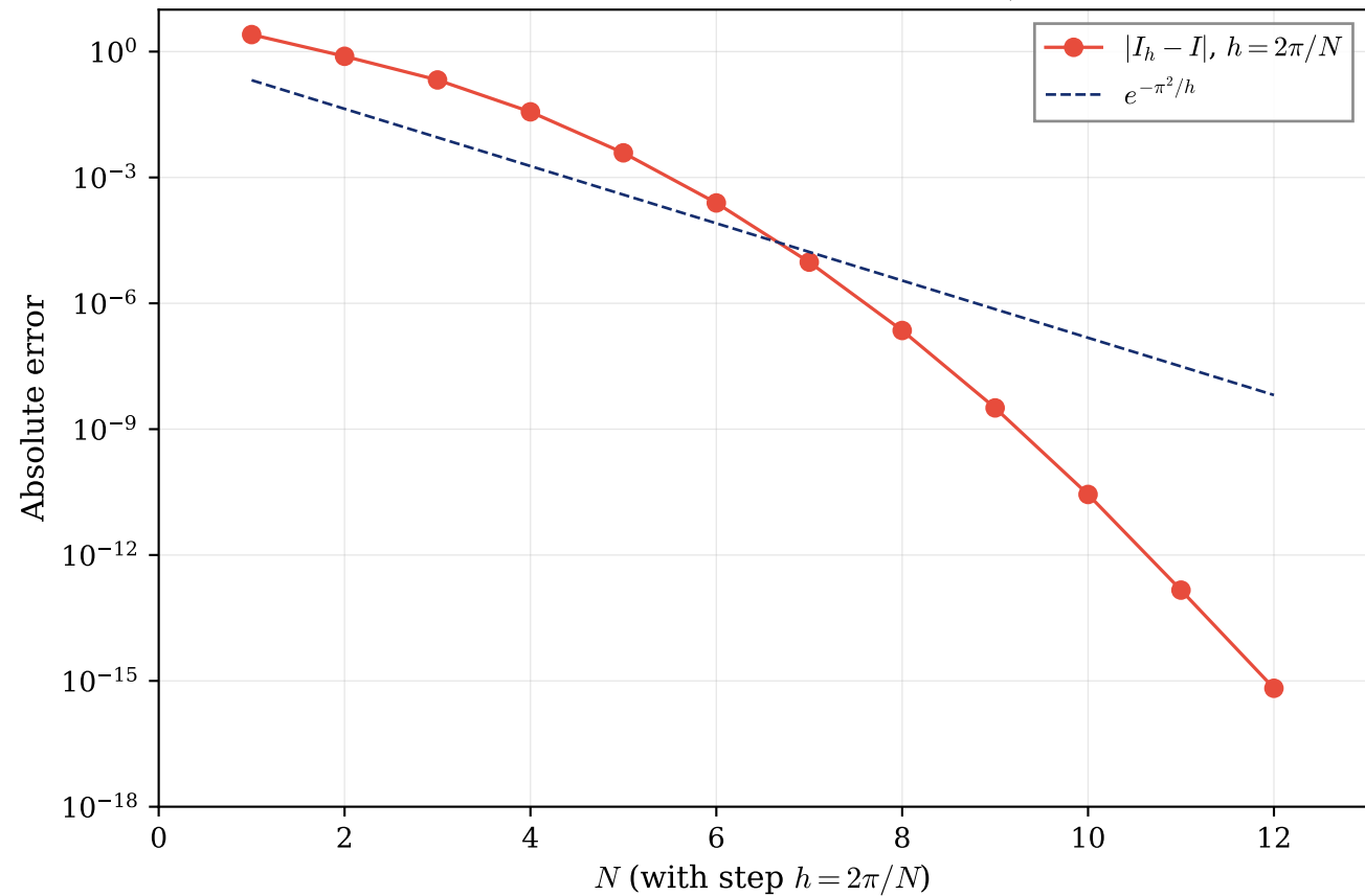
Real-line trapezoidal rule on e^{-x^2}/\sqrt{\pi}
