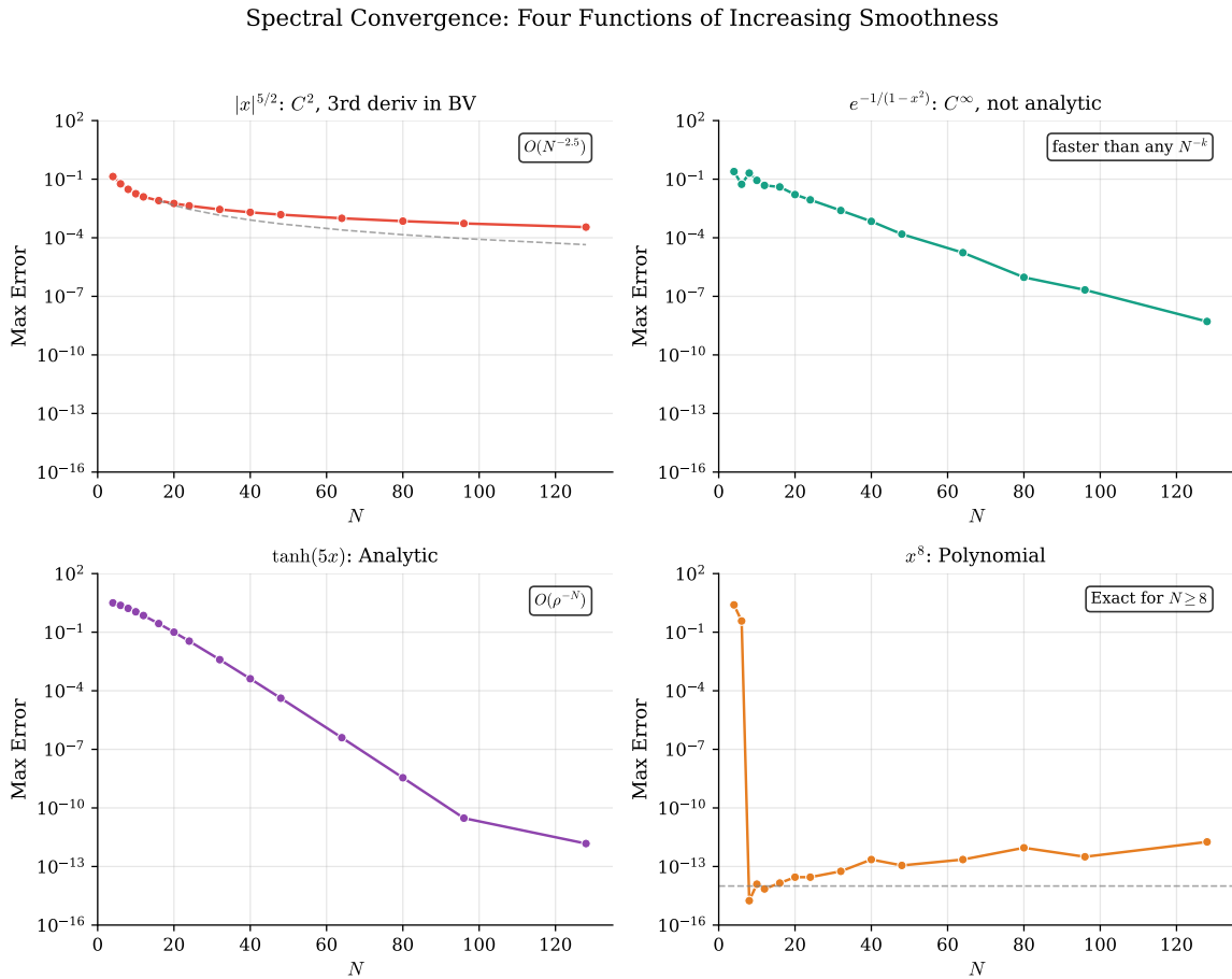
Figure 39: Convergence of the spectral differentiation error \|D_N \mathbf{v} - u'(x)\|_\infty as a function of N for four test functions. Top left: |x|^{5/2} shows algebraic convergence O(N^{-2.5}) due to limited smoothness (Hölder regularity 5/2 ). Top right: the bump function e^{-1/(1-x^2)} achieves superalgebraic (faster than any power) but not exponential convergence, consistent with C^\infty but non-analytic behavior. Bottom left: \tanh(5x) demonstrates exponential convergence until machine precision, as expected for analytic functions. Bottom right: the polynomial x^8 is differentiated exactly for N \geq 8 .
