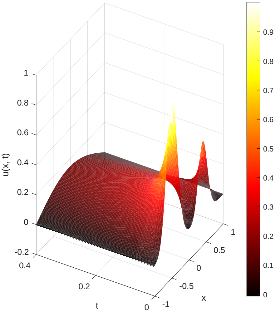
Heat Diffusion: Space-Time View
