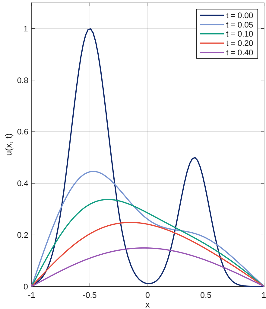
Heat Diffusion: Time Snapshots
