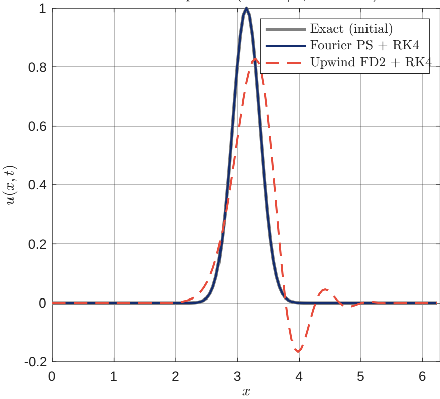
After one period ( t = 2\pi/c , N = 128 )
