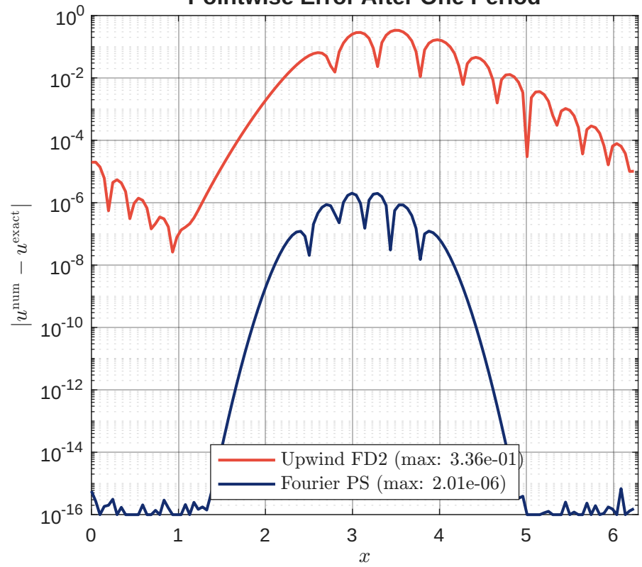
Pointwise Error After One Period
