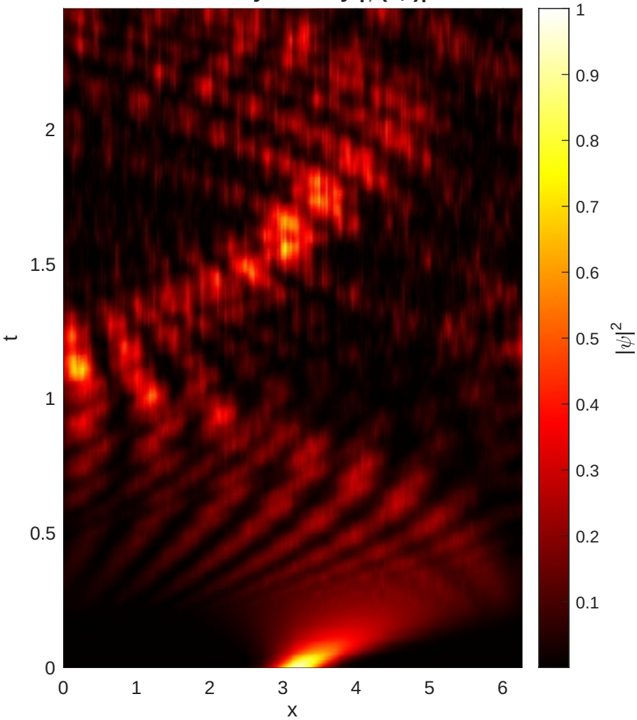
Probability Density |\psi(x,t)|^2
