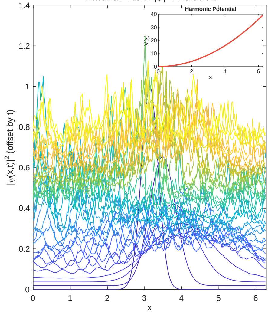
Waterfall View: |\psi|^2 Evolution
