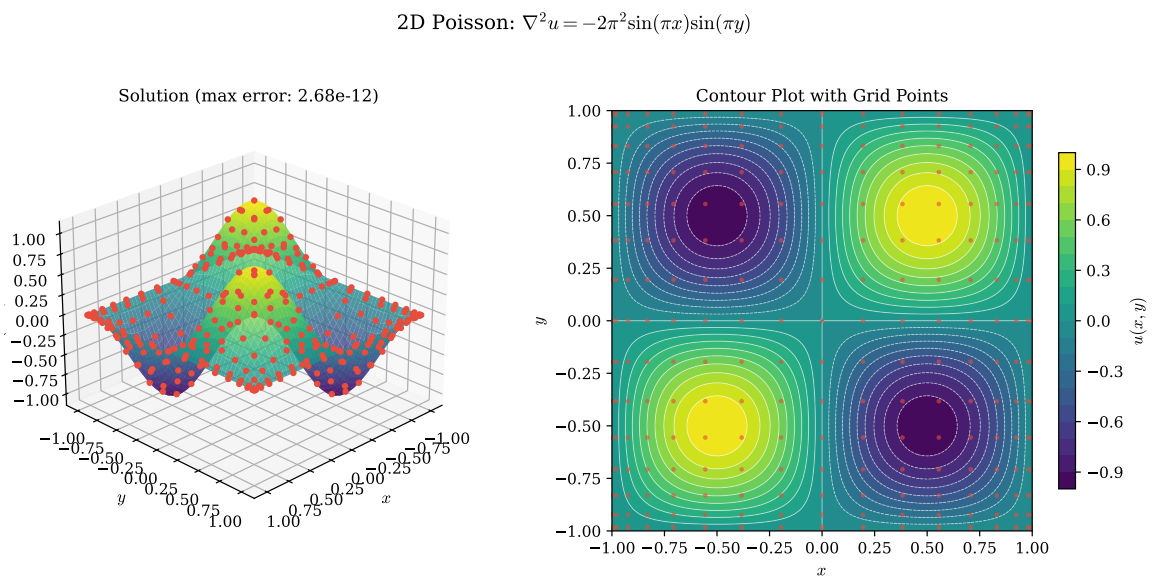
Figure 42: Solution of the 2D Poisson equation Equation 74. Left: 3D surface plot of the solution. Right: contour plot with Chebyshev grid points overlaid. For N = 16 , the maximum error is approximately 10^{-12} .
