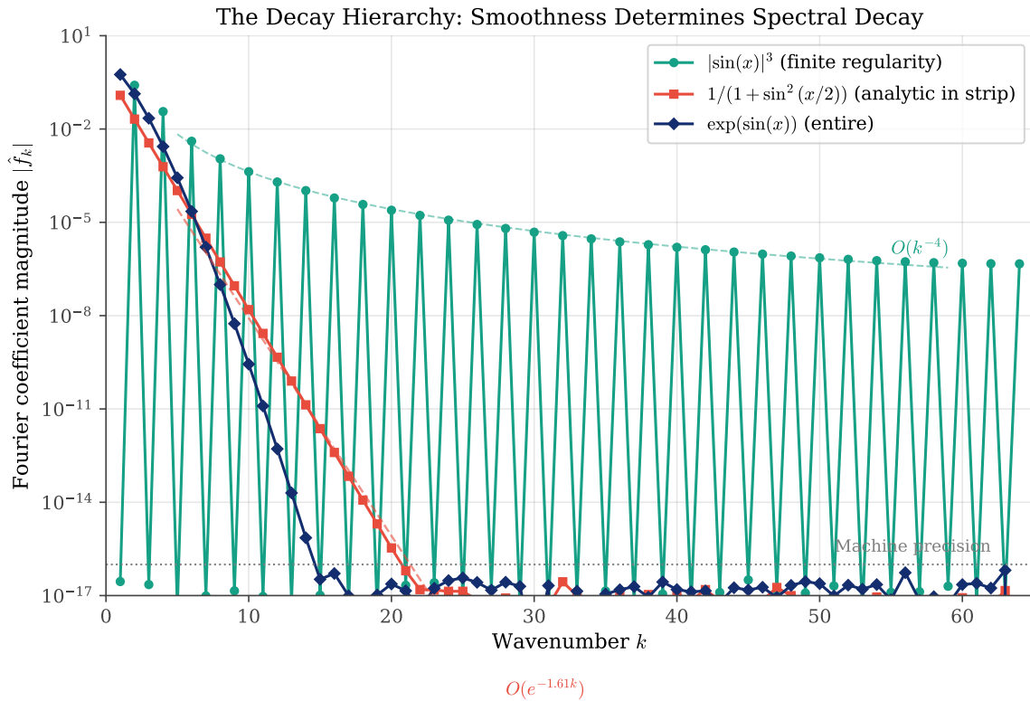
Figure 29: The decay hierarchy of Fourier coefficients. Functions with greater smoothness exhibit faster decay: algebraic ( O(k^{-4}) ) for finite regularity, geometric ( O(e^{-ak}) ) for strip-analytic functions, and super-geometric for entire functions. The plot shows |\hat{f}_k| versus wavenumber k on a semi-log scale.
