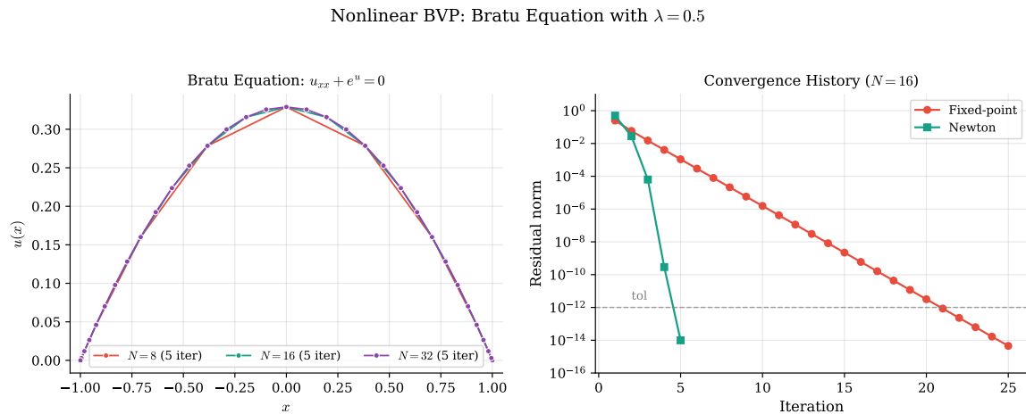
Figure 39: Nonlinear BVP: the Bratu equation Equation 70 with \lambda = 0.5 . Left: solutions for different values of N . Right: convergence history comparing Newton iteration (quadratic convergence) with fixed-point iteration (linear convergence). Newton typically converges in 5–8 iterations.
