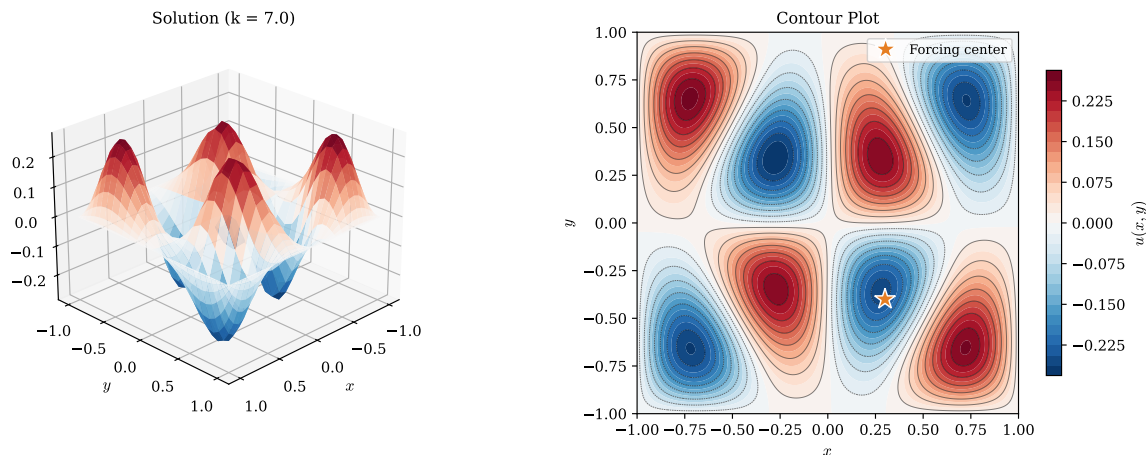
Figure 44: Helmholtz equation Equation 75 with k = 7 , near resonance with the (2,4) eigenmode ( k_{2,4} \approx 7.02 ). Left: 3D surface showing the wave-like structure. Right: contour plot with forcing location marked. The solution exhibits the characteristic pattern of the (2,4) eigenmode.
