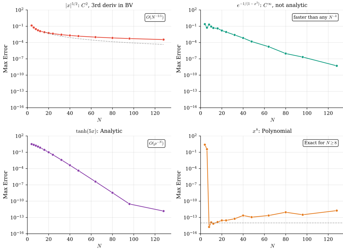
Figure 36: Convergence of the spectral differentiation error \|D_N \mathbf{v} - u'(x)\|_\infty as a function of N for four test functions. Top left: |x|^{5/2} shows algebraic convergence O(N^{-2.5}) due to limited smoothness (Hölder regularity 5/2 ). Top right: the bump function e^{-1/(1-x^2)} achieves superalgebraic (faster than any power) but not exponential convergence, consistent with C^\infty but non-analytic behavior. Bottom left: \tanh(5x) demonstrates exponential convergence until machine precision, as expected for analytic functions. Bottom right: the polynomial x^8 is differentiated exactly for N \geq 8 .
