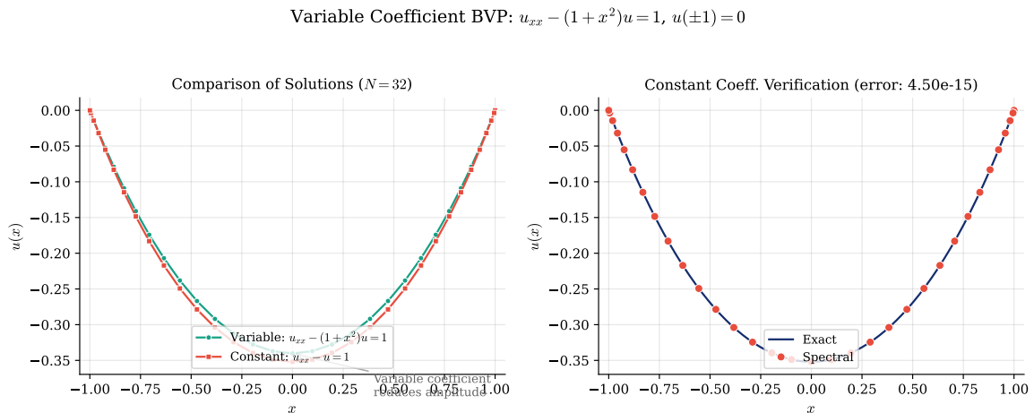
Figure 38: Variable coefficient BVP Equation 68. Left: comparison of solutions for variable coefficient (1 + x^2) and constant coefficient (1). The variable coefficient reduces the solution amplitude, especially near the boundaries where 1 + x^2 is largest. Right: verification of the constant-coefficient case against its exact solution.
