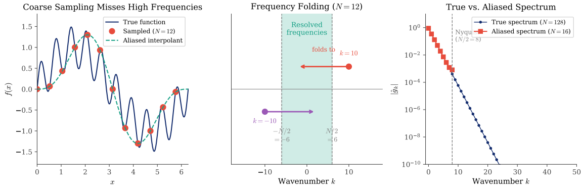
Figure 32: The aliasing phenomenon. Left: A function f(x) = \sin(x) + 0.5 \sin(10x) sampled at N = 12 points. The high-frequency component \sin(10x) aliases to \sin(-2x) , producing a misleading interpolant. Center: Frequency folding diagram showing how wavenumbers k = 10 and k = -10 fold into the resolved range [-6, 6] . Right: True versus aliased spectrum for f(x) = 1/(1.5 + \cos(x)) .
