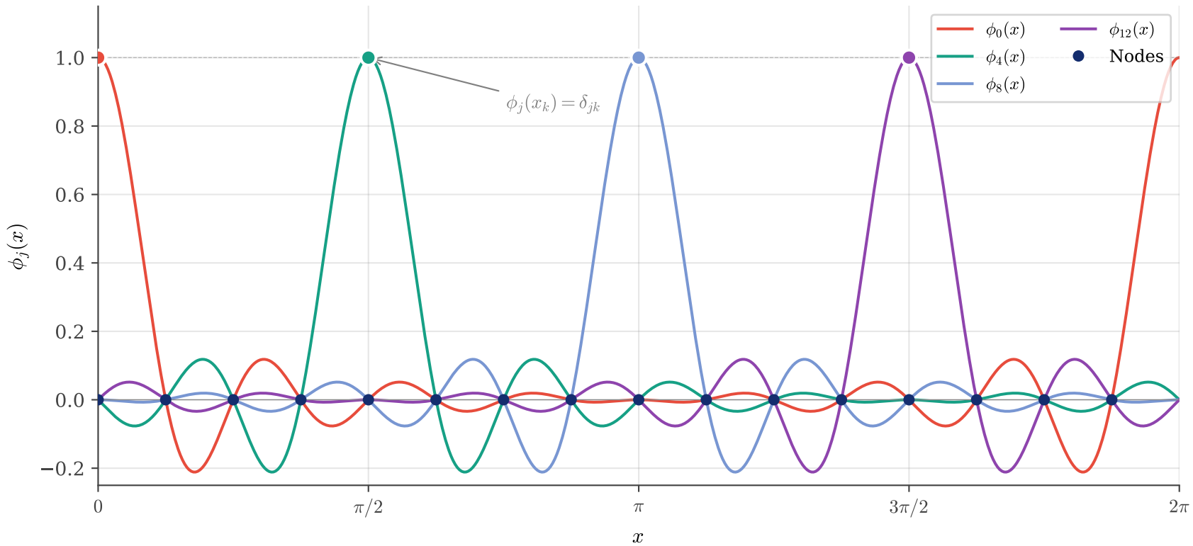
Periodic Cardinal Functions ( N = 16 )
