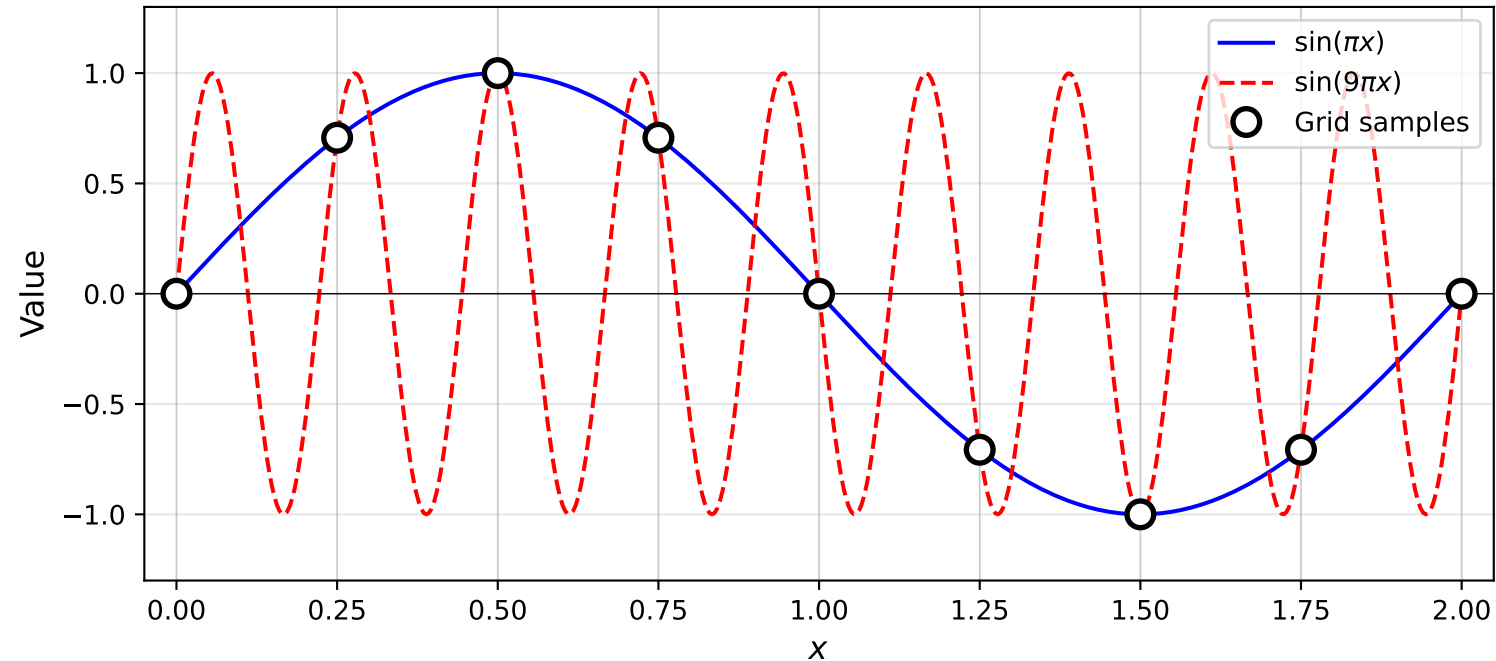
Aliasing on grid h = 1/4 : \sin(\pi x) and \sin(9\pi x) coincide
