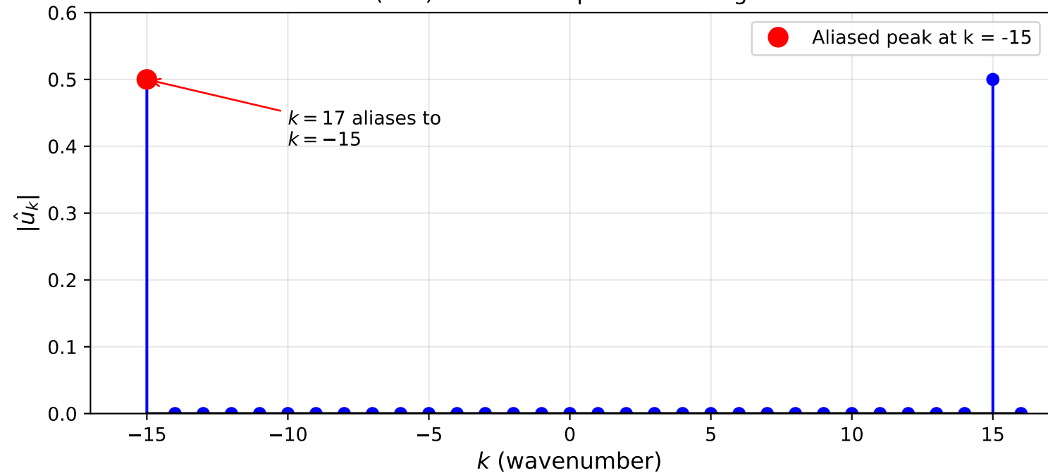
FFT of \sin(17x) with N = 32 points: aliasing to k = -15
