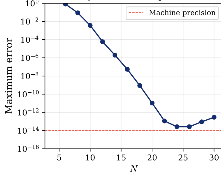
Spectral convergence
