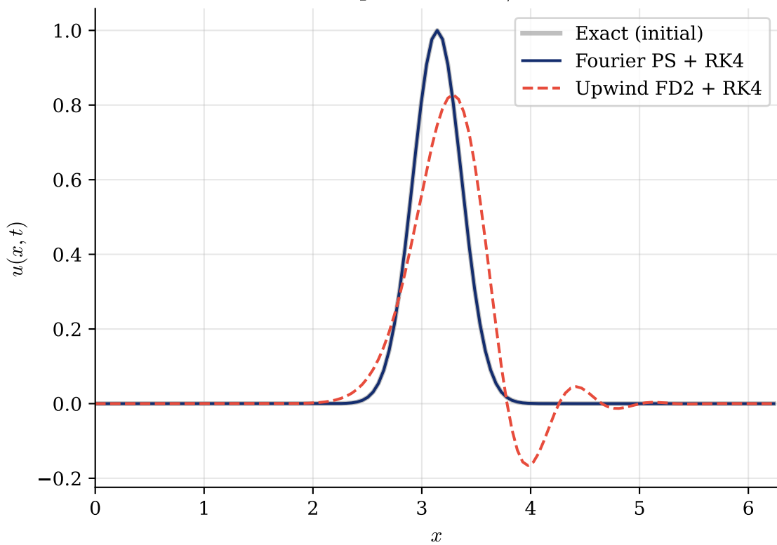
After one period ( t = 2\pi/c , N = 128 )
