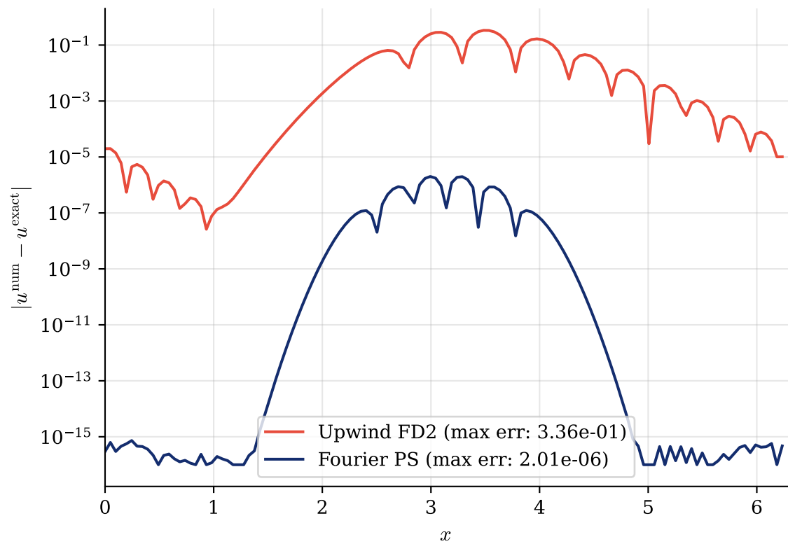
Pointwise Error After One Period
