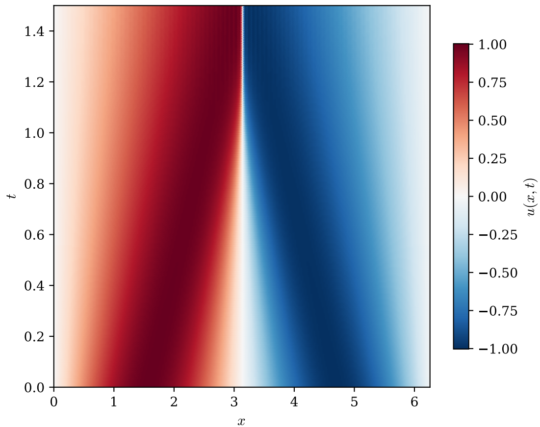
Burgers Equation ( \nu = 0.01 )
