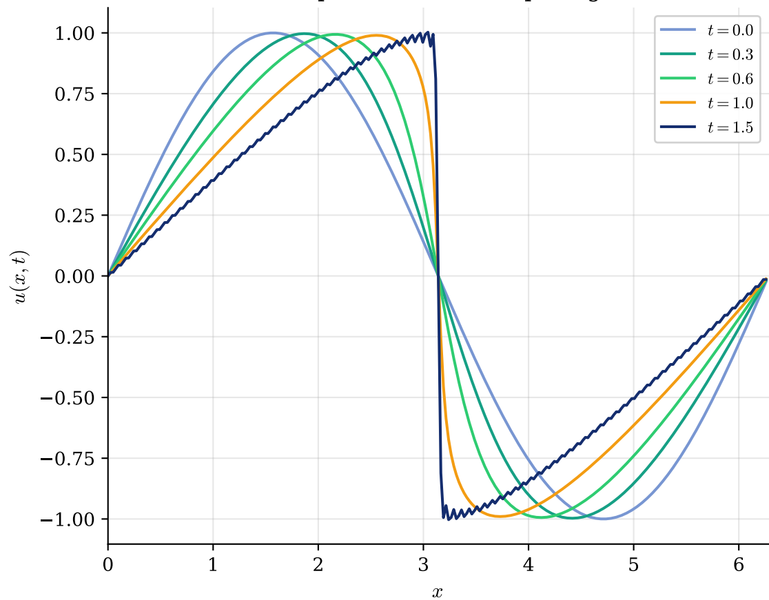
Snapshots: Front Steepening
