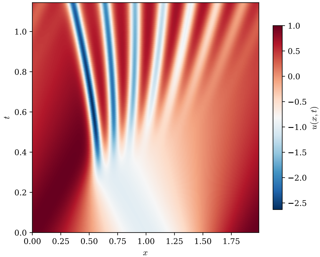
Zabusky--Kruskal Experiment
