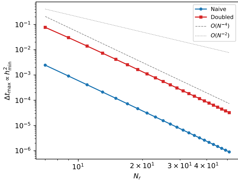
CFL time-step scaling
