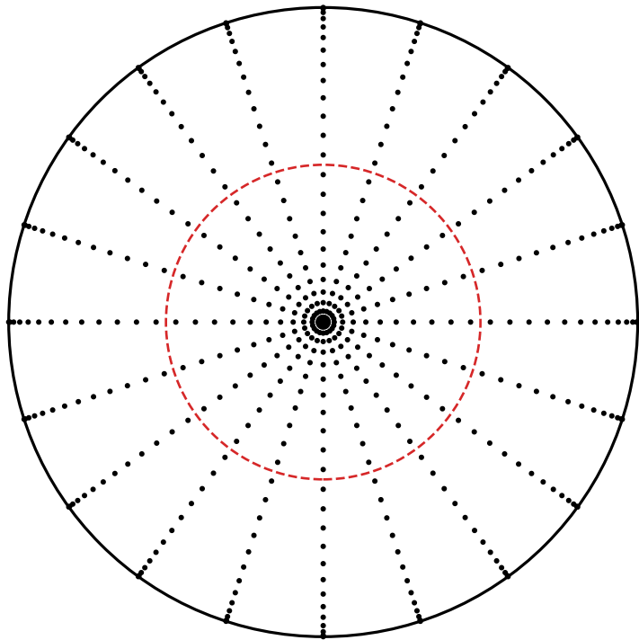
Naive grid ( r \in [0, 1] ) Median circle: 25% of area
