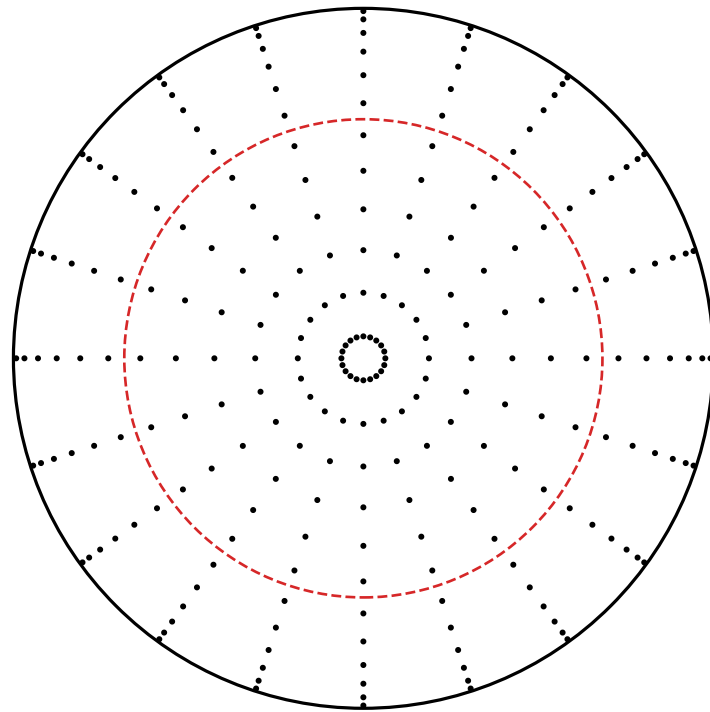
Doubled grid ( r \in [-1, 1] ) Median circle: 47% of area
