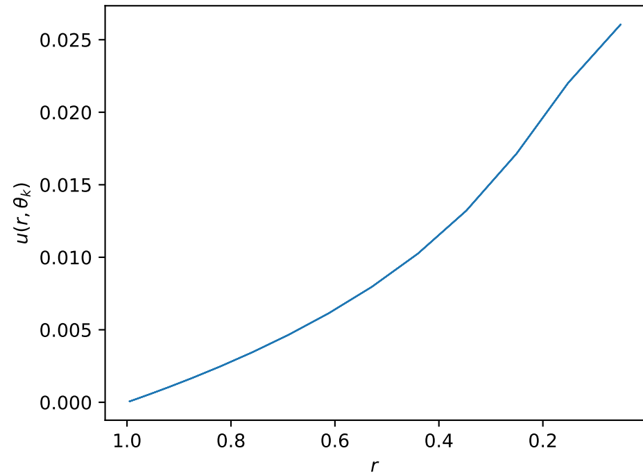
Centred Gaussian: radial profiles (all angles coincide)
