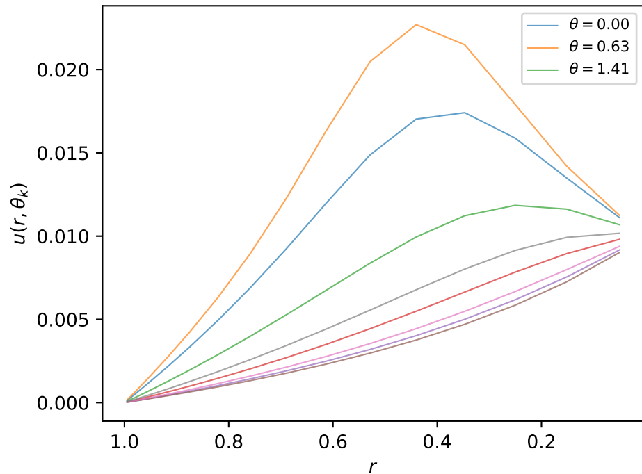
Off-centre Gaussian: radial profiles (angles differ)
