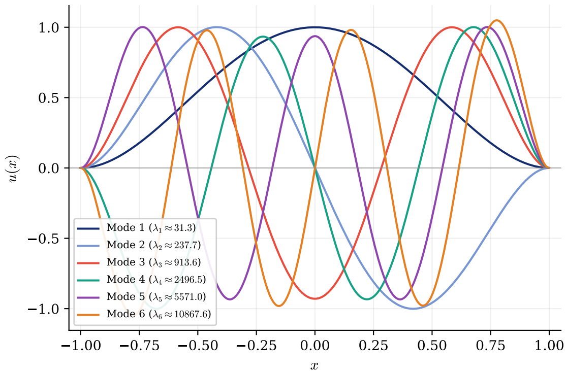
First 6 eigenmodes ( N = 30 )
