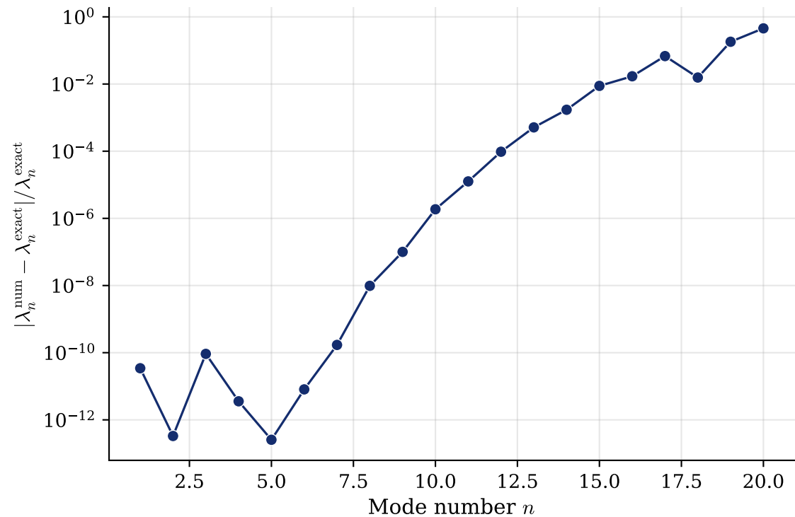
Relative eigenvalue error ( N = 30 )
