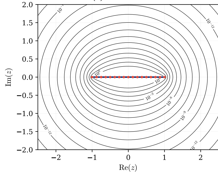
(a) Newton–Cotes
