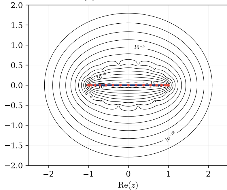
(c) Clenshaw–Curtis
