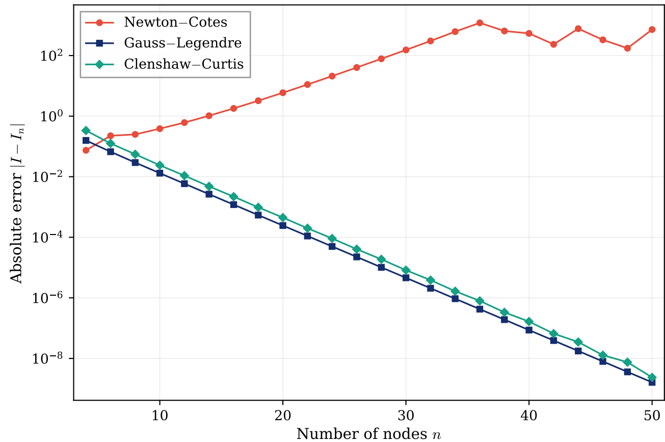
Quadrature of f(x) = 1/(1 + 25x^2) on [-1, 1]
