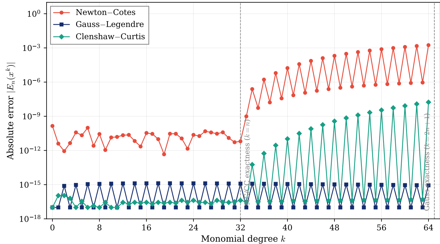
Polynomial exactness of three quadrature rules ( n + 1 = 33 points)
