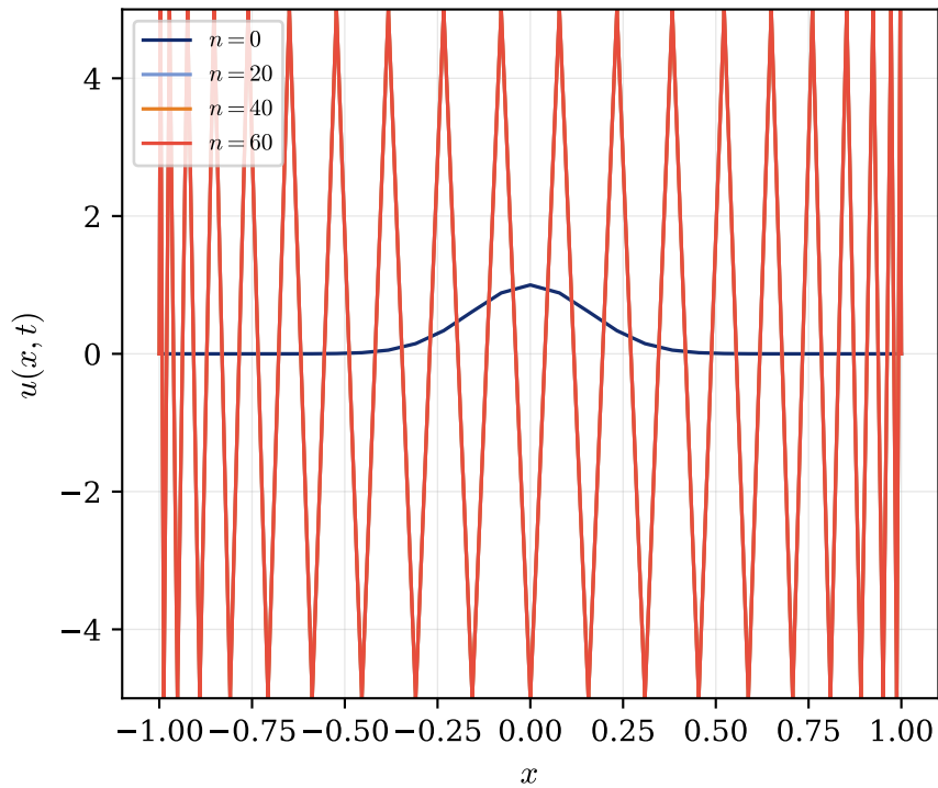
(b) Chebyshev wave, leapfrog
