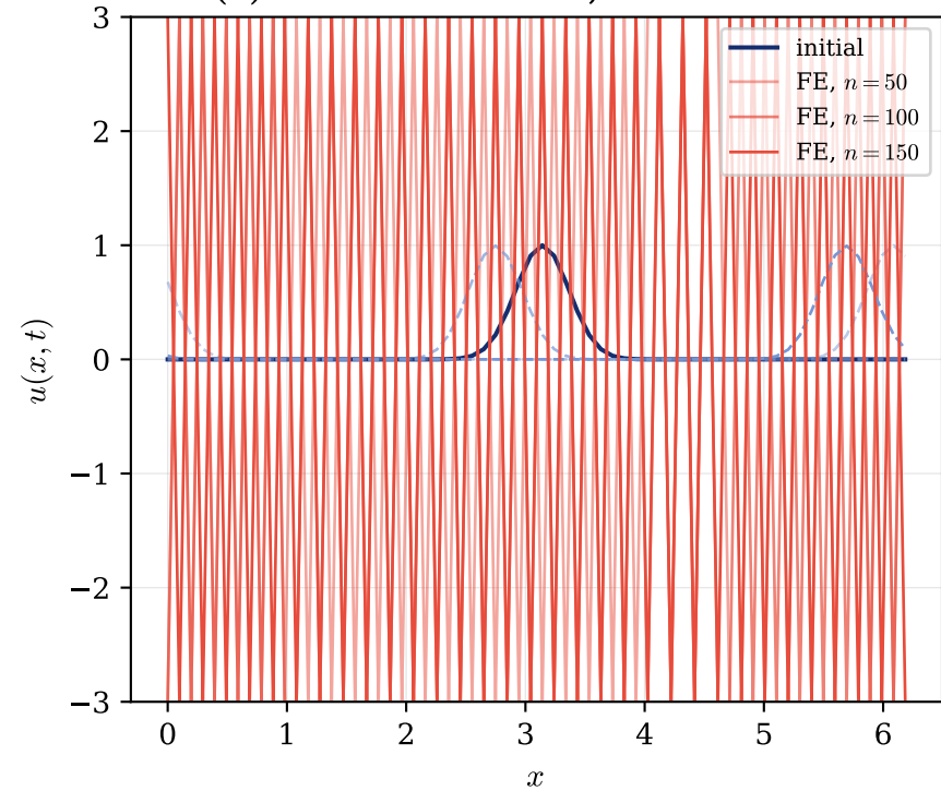
(a) Fourier advection, forward Euler
