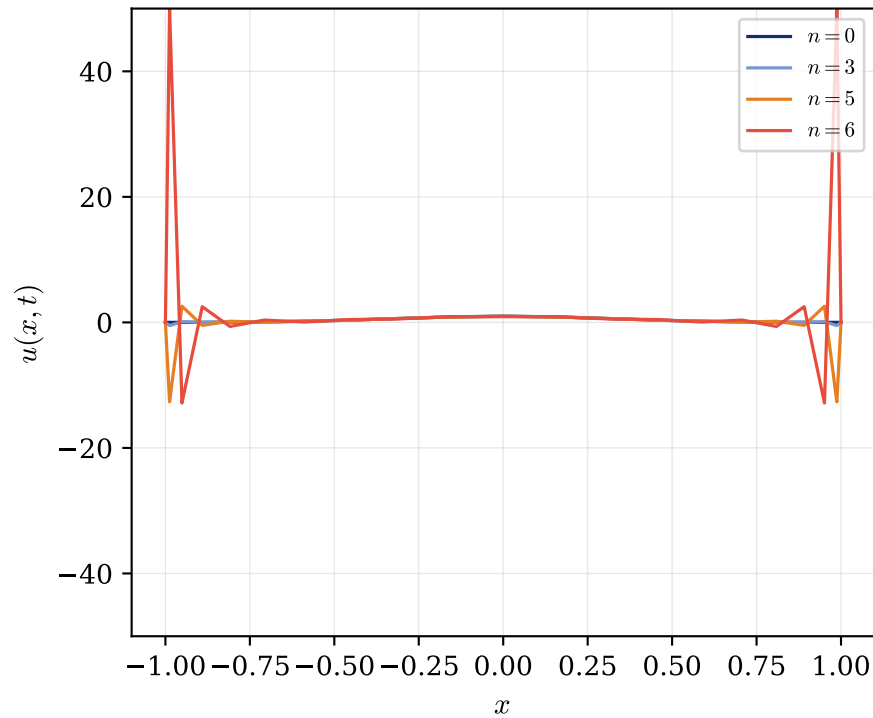
(c) Chebyshev heat, forward Euler
