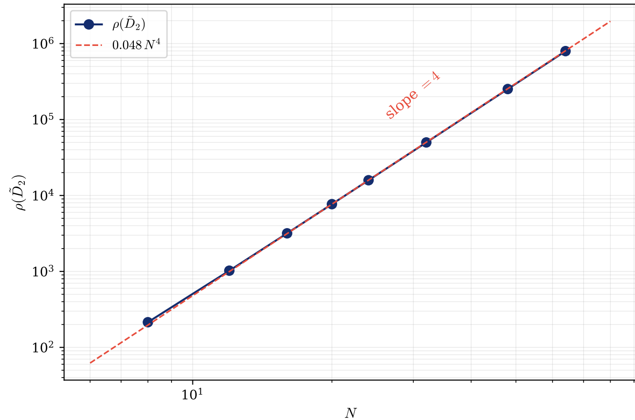
Spectral radius of Chebyshev D^2 (Dirichlet BCs)
