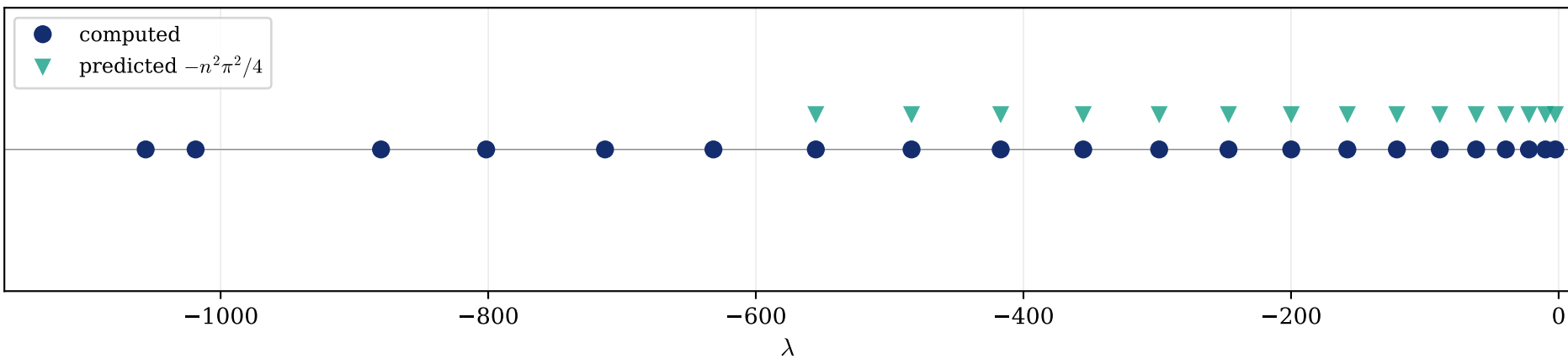
Close-up: physical eigenvalues vs. predicted -n^2\pi^2/4
