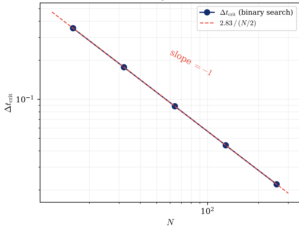
(b) RK4 CFL scaling for Fourier advection
