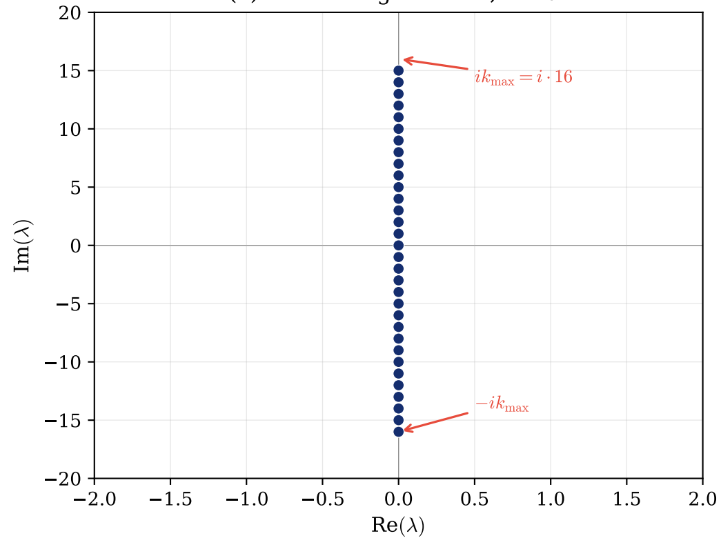
(a) Fourier eigenvalues, N = 32
