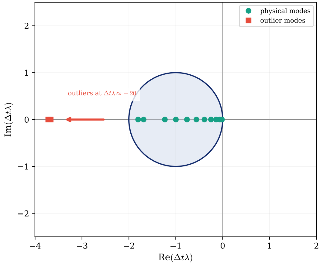
(b) Forward Euler + Chebyshev D^2 ( N=16 )
