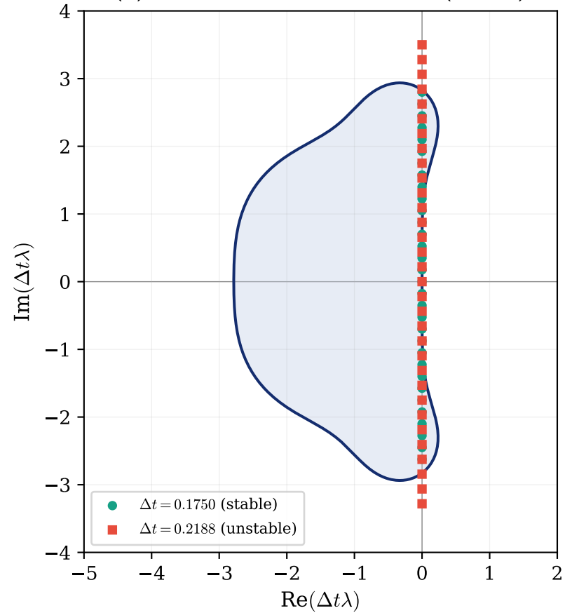
(a) RK4 + Fourier advection ( N=32 )
